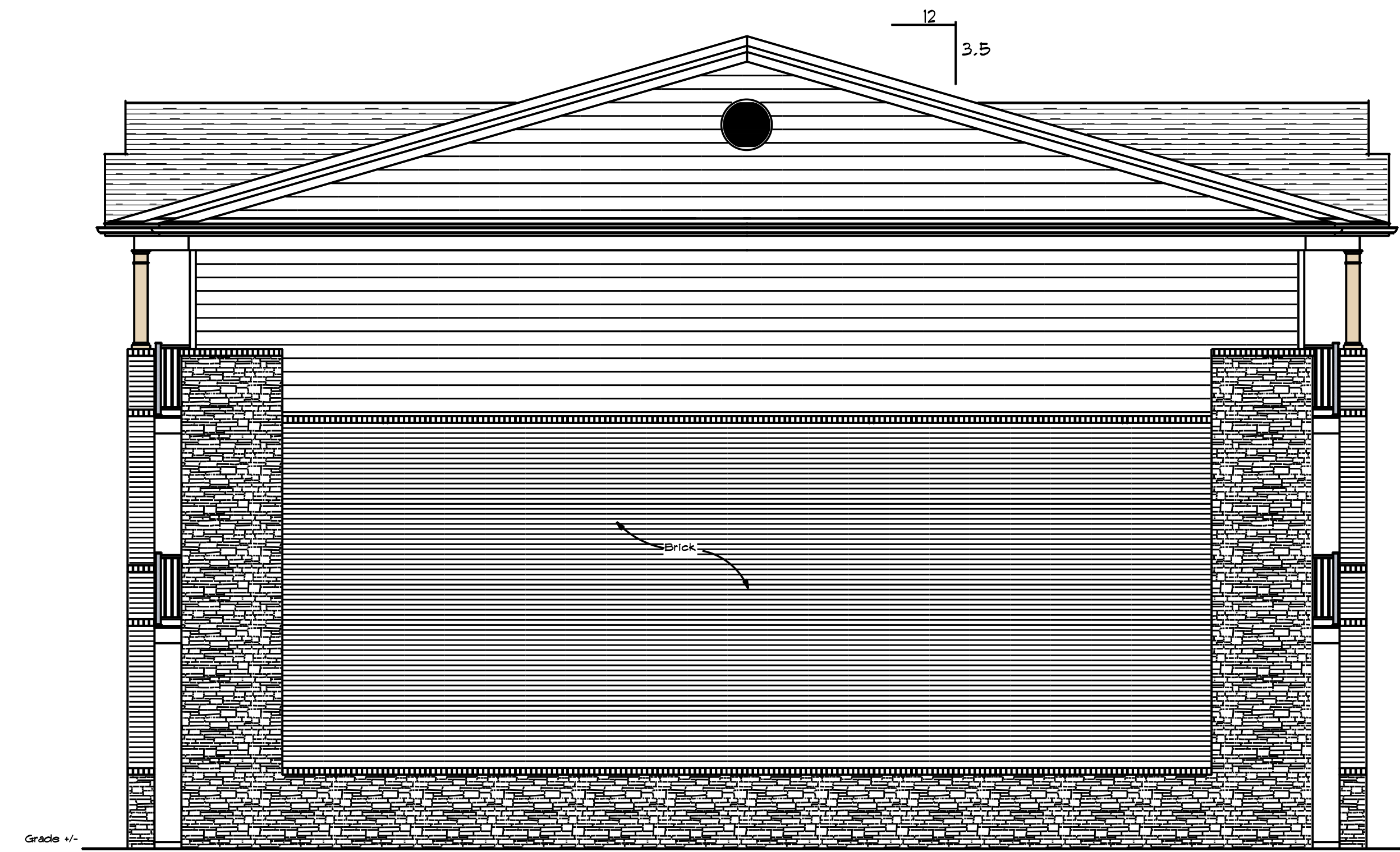
LEFT ELEVATION
