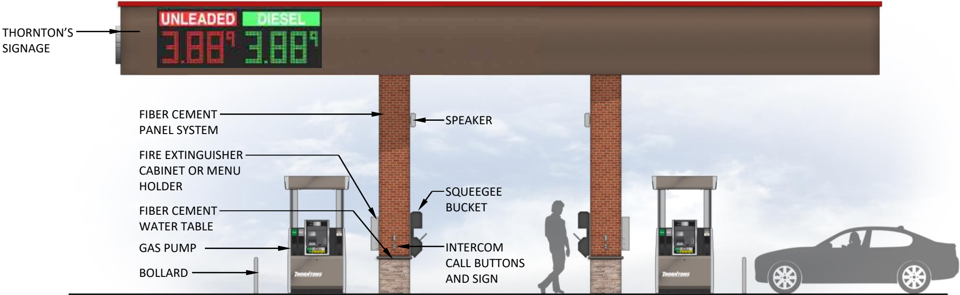
SIDE ELEVATION
