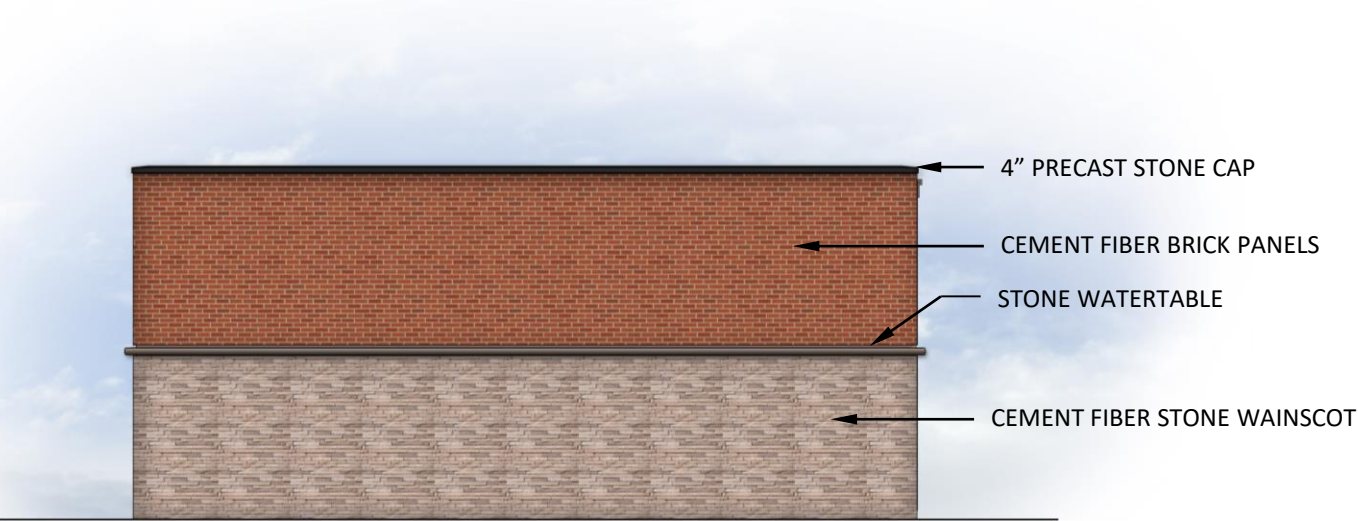
SIDE ELEVATION
