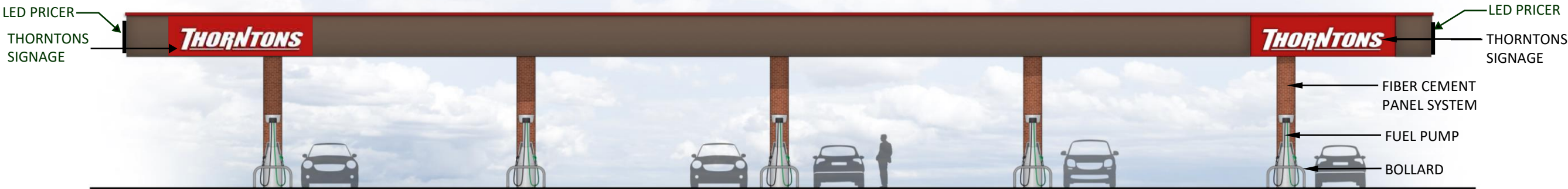
FRONT ELEVATION
