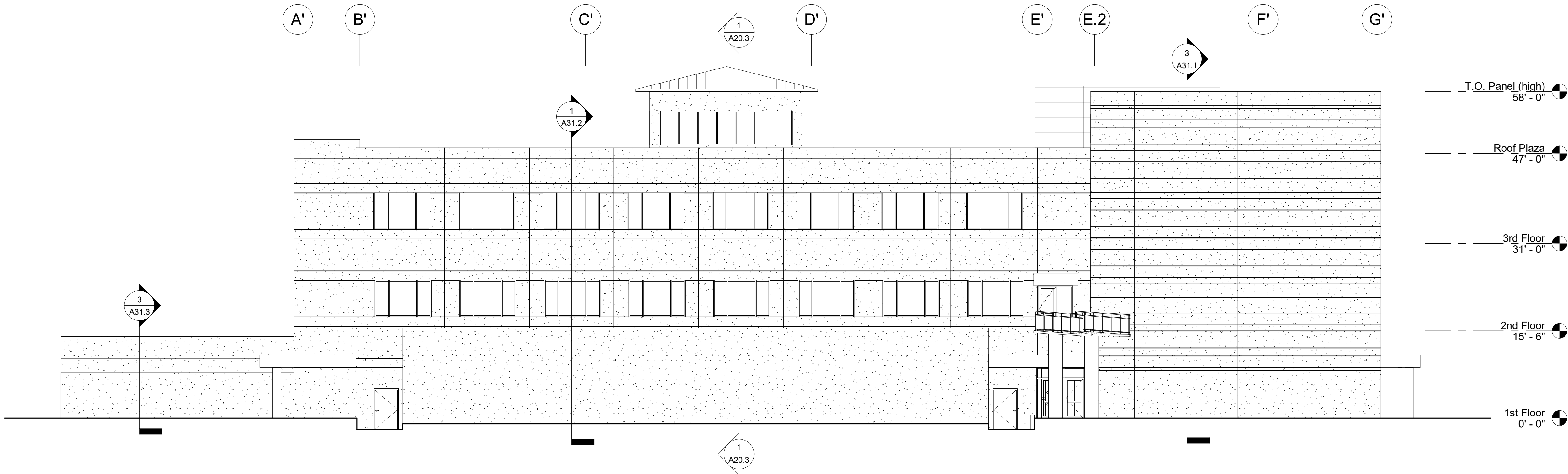
4 North Elevation 3/32" = 1'-0"
