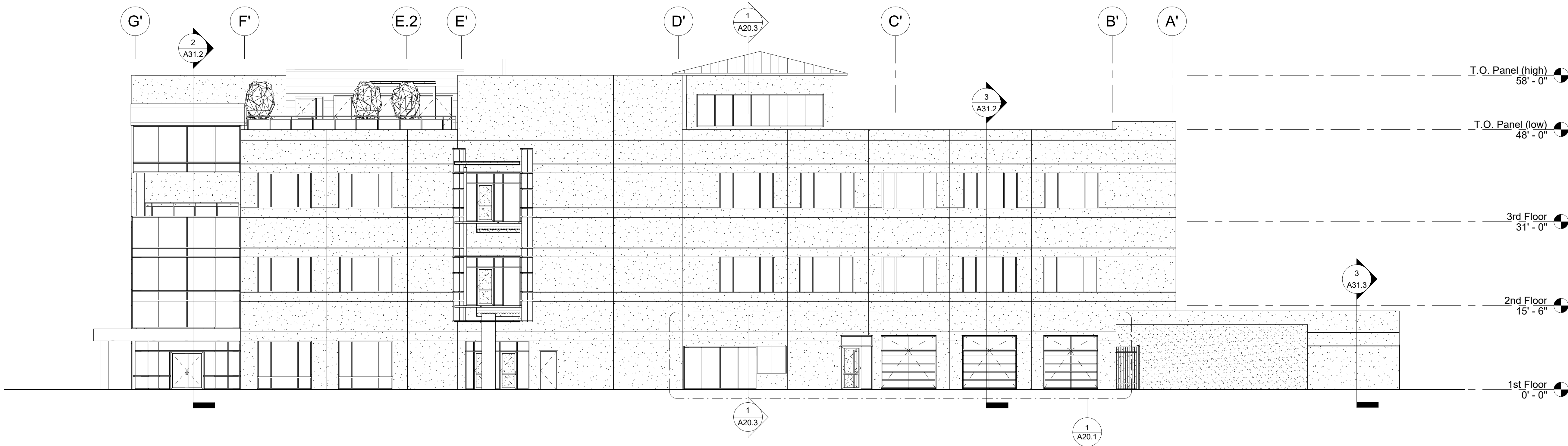
3 South Elevation 3/32" = 1'-0"
