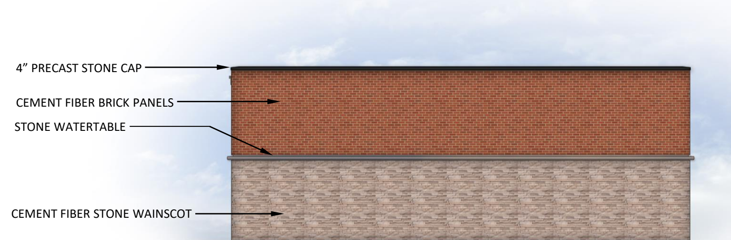
REAR ELEVATION
