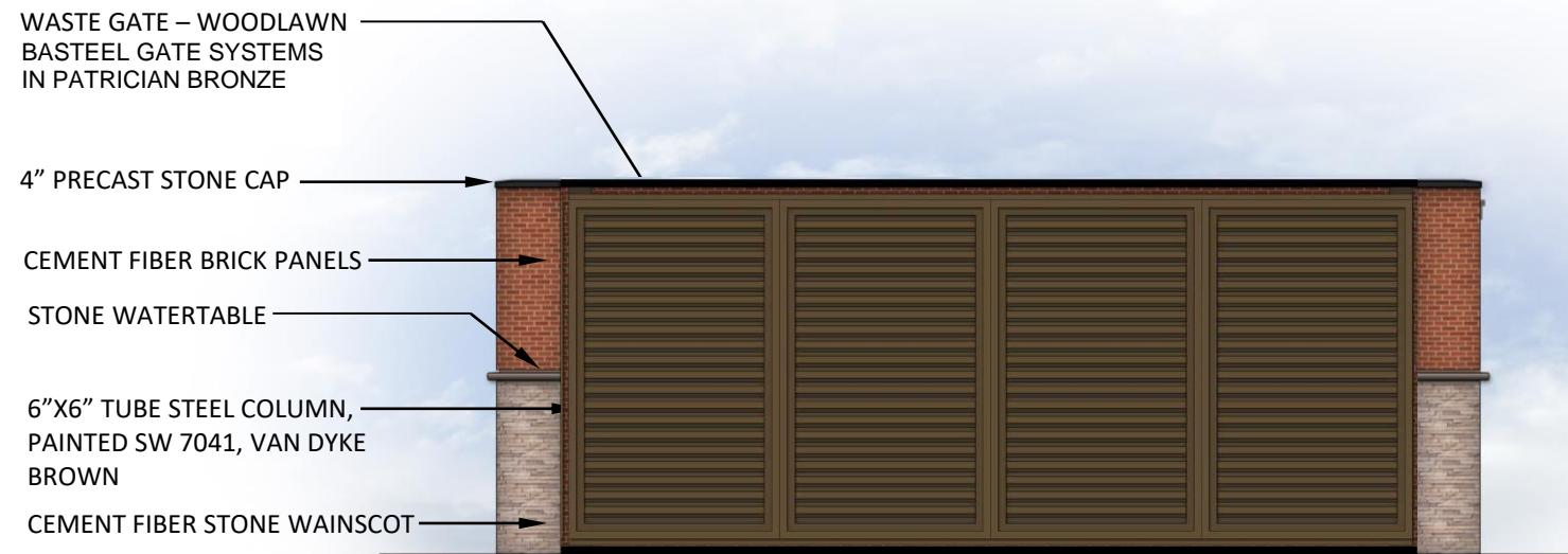
FRONT ELEVATION
