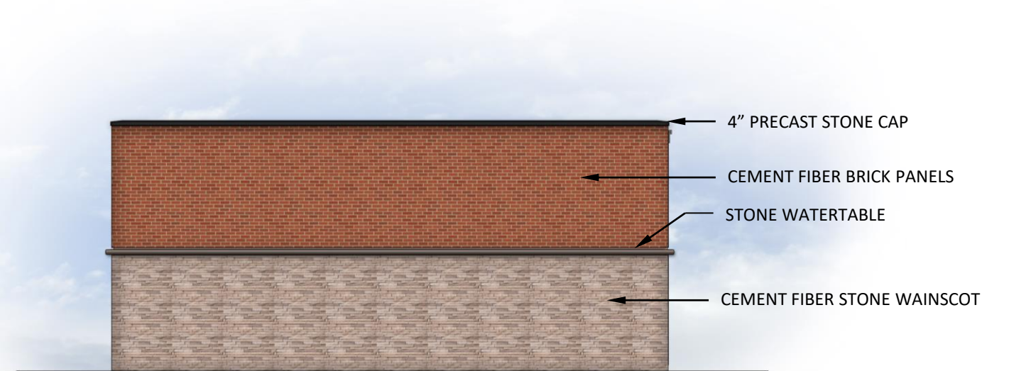
SIDE ELEVATION
